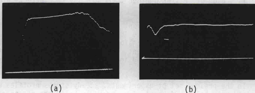
Fig. 2 -- Stress-time profile for shock compression of \text{BaF}_2 in \langle 111 \rangle direction. The impact stress in both cases is 40 kbars. (a) The profile recorded on Tektronix Type 454 oscilloscope. (b) The profile recorded on Tektronix Type 519 oscilloscope.
